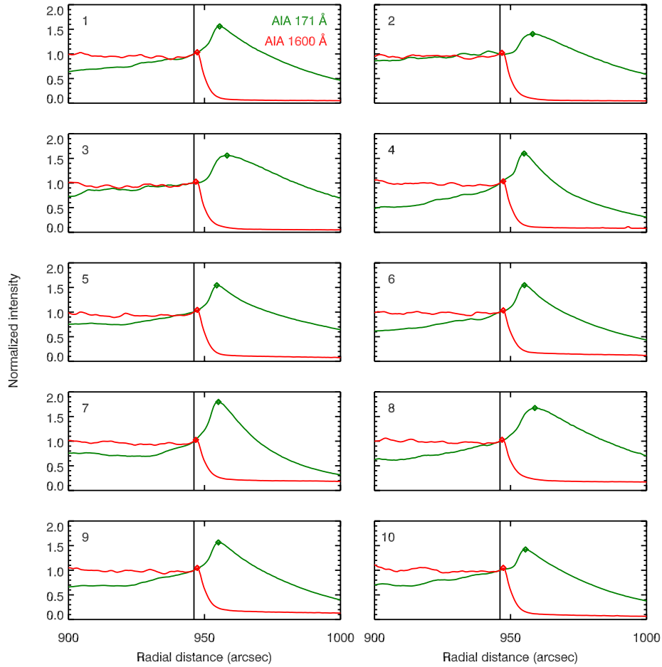
Figure 14. Limb positions in the AIA full-disk data. We show the intensity as a function of radial distance across the limb averaged in the azimuthal direction (i.e. along the limb) for the ten limb segments marked in Fig. 13. The red lines are for the 1600 Å channel, the green lines for the 171 Å band. The dots mark the respective limb positions defined as the local maximum before the intensity drops above the limb. The radial distance is measured from disk center. See Appendix A.
