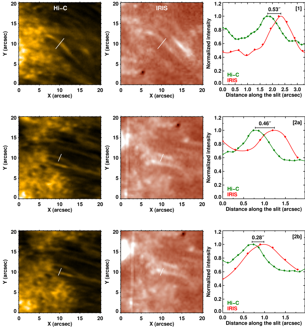
Figure 5. Spatial offset between loops seen in Hi-C and IRIS. The left and middle panels show zooms into the Hi-C and IRIS images centered around the features as marked in Fig. 4. The top row shows the loop feature [1] the middle and bottom row the two parts of the double feature [2], here marked [2a] and [2b]. In the respective right panel we display the variation of the intensities in Hi-C and IRIS along the white lines (strips) marked in the respective left panels, i.e. roughly perpendicular to the loop. The diamonds show the data interpolated onto the plate scale of the respective instrument, the solid curves show interpolations at higher resolution to measure the offsets between the two instruments. The offsets between Hi-C and IRIS are marked with the plots. The typical error for the offsets is 0.1'' . See Sect. 4.2.
