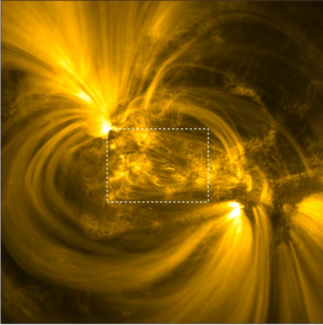
Figure 3. Hi-C image showing warm loops in a solar active region. This displays emission around 172 \text{ \AA} seen by Hi-C over its full field of view of 265'' \times 265'' at 19:00:33 UT on May 29, 2018. The center of the image is about 114'' east and 259'' north of disk center. The rectangle marks the core of the active region with the abundant small loops. This 83'' \times 60'' sub-region is imaged in more detail in Fig. 4.
