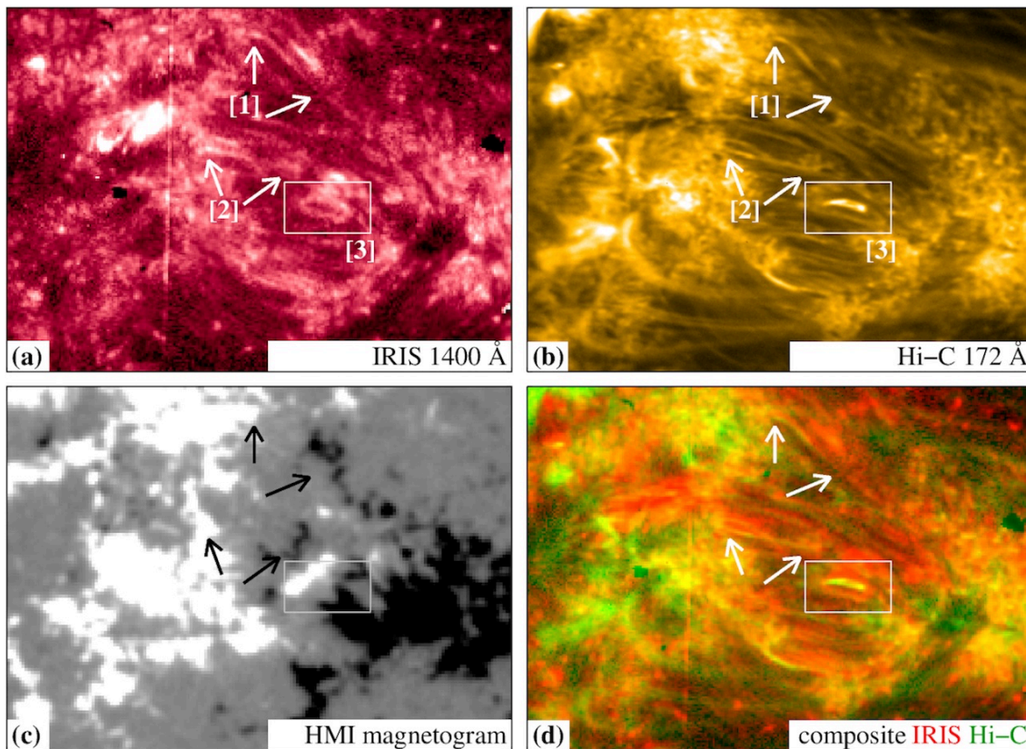
Figure 4. Core of the active region. The field of view of each panel is 83'' \times 60'' and corresponds to the rectangle in Fig. 3. Panels (a) and (b) show the images in the IRIS 1400 Å channel and in Hi-C 172 Å. To highlight fainter structures, the IRIS image is on a logarithmic scale, the Hi-C image is scaled with a power of 0.3. The multi-color composite of these two bands is displayed in panel (d), with green for Hi-C and red for IRIS data. For context, in panel (c) we display a co-temporal magnetogram acquired by HMI showing the line-of-sight component of the magnetic field in the photosphere ( \pm 200 G). The footpoints of features [1] and [2] are indicated by the arrows. The rectangle highlights the peculiar small loop [3] that is briefly discussed in Appendix C. The Hi-C image shown here was taken at 19:00:33 UT, the IRIS and HMI data are those available closest in time. North is top and west is right.
