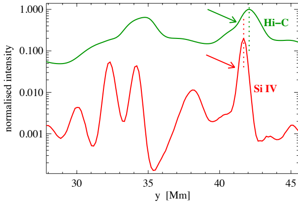
Figure 11. Cut through cool and warm loops in the 3D MHD model. This shows the intensity variation in Si IV and Hi-C along the yellow line in Fig. 10. The offset between the loops in Si IV and Hi-C near y \approx 42 Mm is about 400 km. These loops are highlighted by arrows and are the same as pointed to in Figs. 10 and 12. See Sect. 6.2.
