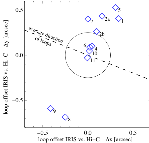
Figure 18. Offsets between loops in Hi-C and IRIS. Each diamond represents one feature labeled in the same scheme as in Fig. 5, Fig. 16 and Table 1. The dashed line shows the average direction of the loops (cf. Fig. 4b) reflecting the overall orientation of the magnetic features. The circle has a diameter of 0.5'' that is a slightly larger than the resolution of either Hi-C or IRIS. See Appendix B.
