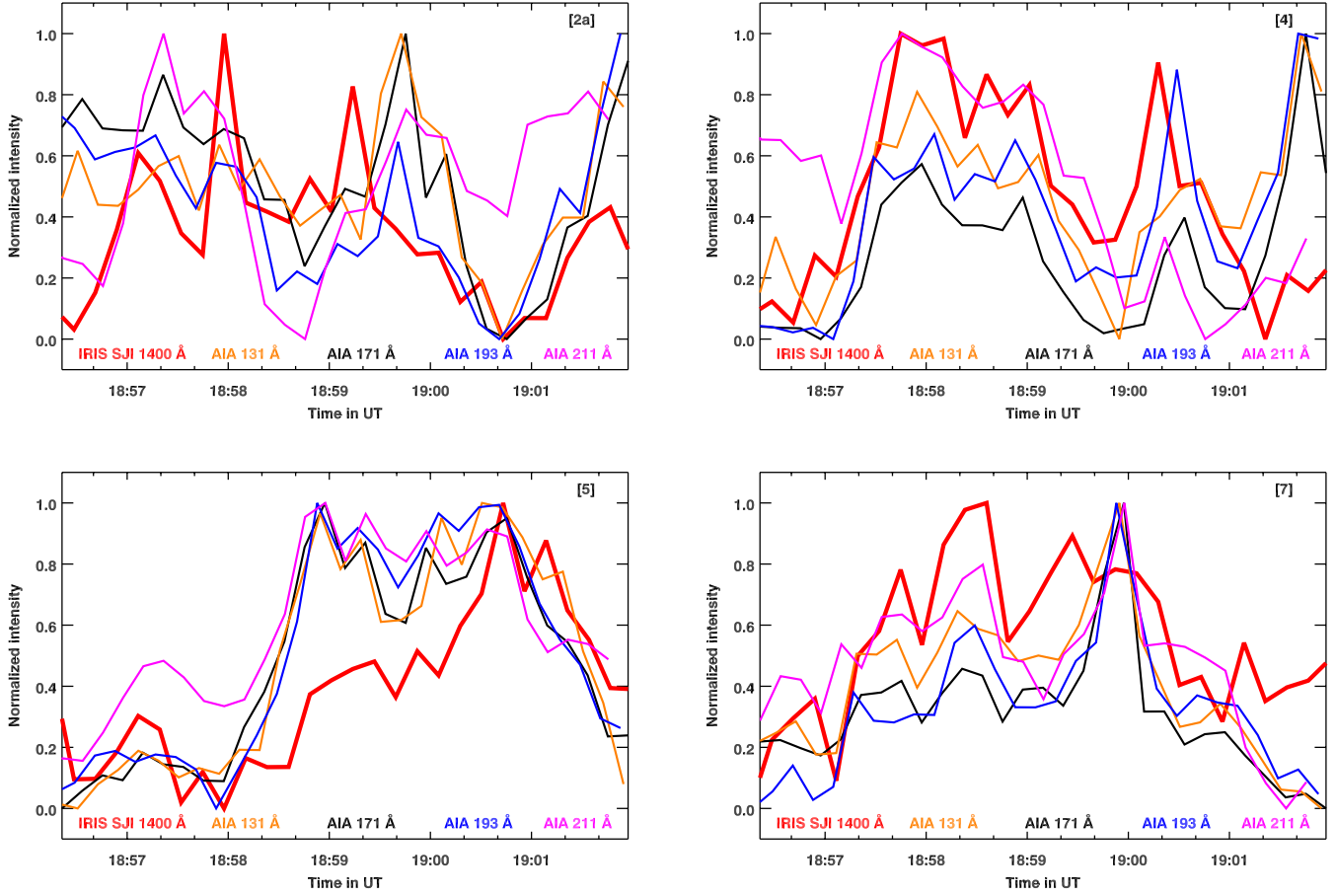
Figure 8. Temporal evolution of selected loops. Each panel shows the light curves for one loop example for four AIA channels and the IRIS 1400 Å images. The number of each feature is given in the top right corner of each panel. The temperature contributions (or kernels) of these AIA channels and the Si IV line are displayed in Fig. 9. The labels in the panels refer to the features shown in Figs. 5 and 16. In order not to overcrowd the panels, we do not show the light curves in the Hi-C 172 Å band which are almost exactly the same as for the AIA 171 Å channel. All light curves are normalized by mapping the respective minimum and maximum values to the range of [0,1]. See Sect. 5.1 and Appendix D.3.
