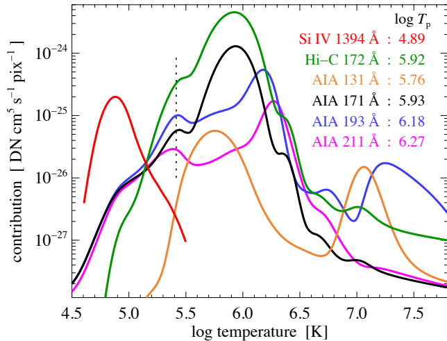
Figure 9. Contribution functions for Hi-C, AIA and Si IV. The response functions for the (selected) AIA channels are calculated using the routines available in SolarSoft ( http://www.lmsal.com/solarsoft/ ). The corresponding curve for Hi-C is from the Hi-C instrument paper (Rachmeler et al. 2019). The contribution function for the Si IV line is calculated using Chianti (Dere et al. 2019) and is scaled to fit on this plot. For each of the curves the temperature T_p of the peak of the contribution function is listed with the legend as \log_{10} T_p [K]. The dotted line indicates a temperature of 0.26 MK. See Sect. 5.2.1 and Appendix D.2.
