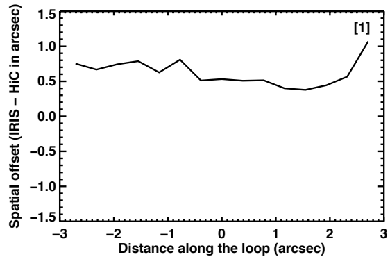
Figure 6. Offset between loop in Hi-C and IRIS data. This shows the offset along feature [1] pointed to in Fig. 4 and shown in Fig. 5. The distance 0'' along the loop is at the location in Fig. 5[1] where the white slit crosses the loop. The offset between Hi-C and IRIS is consistently to the same side. See Sect. 4.3.
