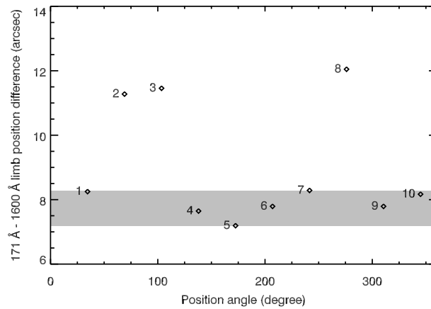
Figure 15. Offset of the limb position between the AIA 171 Å and 1600 Å images. The numbered diamonds show the difference of the limb position between the two bands as derived from the respective intensity variations in Fig. 14 in the segments marked in Fig. 13. The grey band indicates the standard deviation around the mean value (discarding segments 2, 3, and 8 are within the polar coronal holes). See Appendix A.
