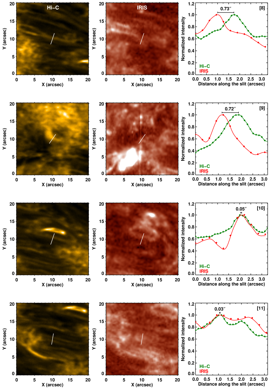
Figure 17. Further examples for offsets. Same as Fig. 16, but for cases [8–11] in Table 1. See Appendix B.
