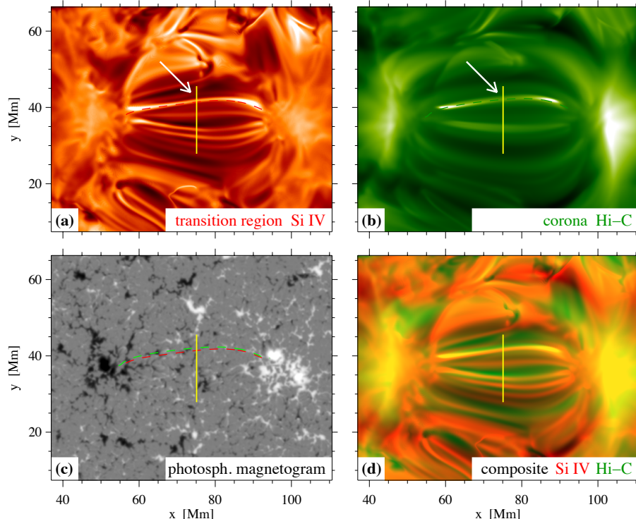
Figure 10. View of the 3D MHD model from straight above. The layout is similar to the observations in Fig. 4. Panels (a) and (b) show the emission originating from Si IV, similar to the IRIS 1400 Å image, and from Hi-C. Both the Si IV and Hi-C intensity have been integrated vertically through the computational domain. Panel (c) shows the vertical component of the magnetic field in the photosphere of the simulation. The multi-color composite of the cool and warm emission is displayed in panel (d). Here the red channel represents Si IV, the green channel Hi-C. The field of view covers only about one quarter of the horizontal extent of the 3D MHD model. The red and green dashed lines show the projection of magnetic field lines passing through the center of the loops seen in Si IV and Hi-C (traced in the 3D data cube). The vertical yellow lines shows the location of the cuts in intensity shown in Fig. 11 and of the vertical cuts in Fig. 12. The arrows in panels (a) and (b) point to the respective loop in Si IV and Hi-C highlighted also by arrows in Figs. 11 and 12. See Sect. 6.2.
