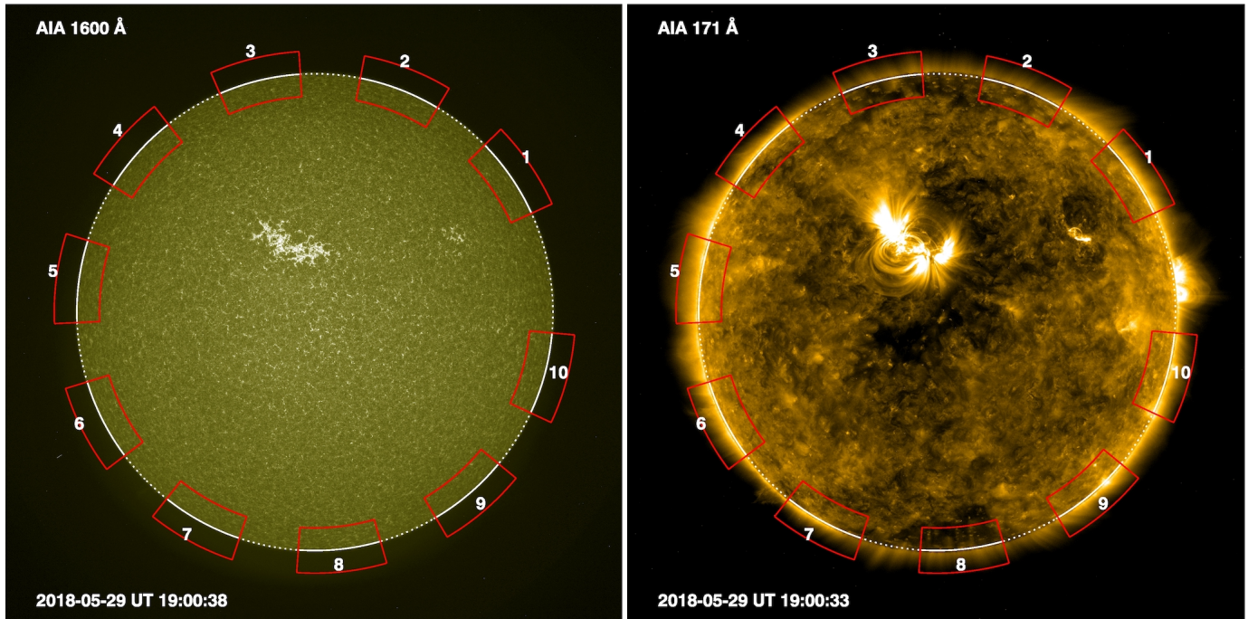
Figure 13. Full-Sun images acquired by AIA in its 1600 Å and 171 Å channels. The solid/dotted lines show the limb through a circle with the solar radius as recorded in the header of the AIA 171 Å image. The segments numbered 1 to 10 mark the regions to verify the limb alignment between the two channels. Segments 2, 3, and 8 are at locations where (polar) coronal holes are present. The coronal holes are revealed by lower intensities in the 171 Å image. The target region of the Hi-C campaign is the bright active region north-east (top-left) of disk center. See Appendix A.
