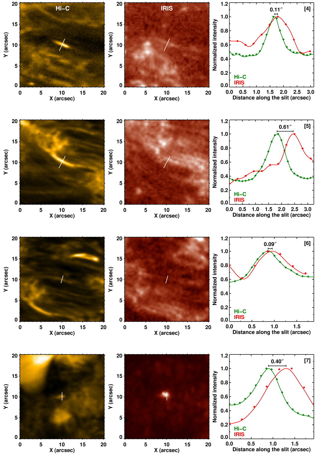
Figure 16. Examples [4] – [7] of loops with spatial offsets between Hi-C and IRIS. The panels have the same format as used for the features in Fig. 5. For each feature the left panels shows a zoom into the Hi-C and IRIS images with the white line marking the cut. The respective right panel shows the intensities in Hi-C (green) and IRIS (red) across the loop along the cut. The diamonds show the data interpolated on the plate scale of the respective instrument, the solid curves show interpolations at higher resolution to measure the offsets between the two instruments. The offsets are indicated with the plots and are listed in Table 1. The typical error for the offsets is 0.1'' . The distance along the slit is counted positive towards the northern (large values of Y) tip of the cut. See Appendix B.
