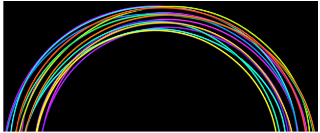
Figure 2. Internal braiding of a bundle of fieldlines in a loop. The braided magnetic field lines are shown in different colours. They are based on a 3D MHD model similar to Pontin et al. (2017) where the magnetic field started to relax. While the original model is for a straight loop, here we curved the appearance to resemble a semi-circular loop. See Sect. 2 for details.
