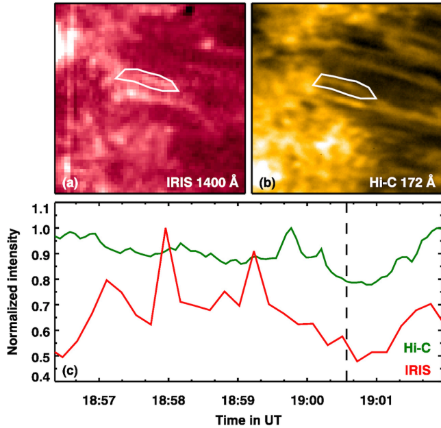
Figure 7. Spatio-temporal evolution of the intensity in one selected loop feature. Panels (a) and (b) show a zoom of the IRIS 1400 Å and Hi-C 172 Å channels into feature [2a] identified in Fig. 4. Panel (c) displays the temporal evolution in part of the respective feature integrated over the polygons indicated in the top panels. These polygons encompass 74 and 514 pixels in the cases of IRIS and Hi-C, respectively. The light curves in Hi-C (green) and IRIS (red) are shown in normalized to their peak value. The peak counts are about 3600 DN for IRIS and 3.4 \times 10^6 DN in Hi-C. The dashed line in panel (c) indicates the time the images in panels (a) and (b) are recorded. A movie showing the temporal evolution is available online ( http://www2.mps.mpg.de/data/outgoing/peter/papers/2019-hic/movie-s1.mp4 ). See Sect. 5.1.
